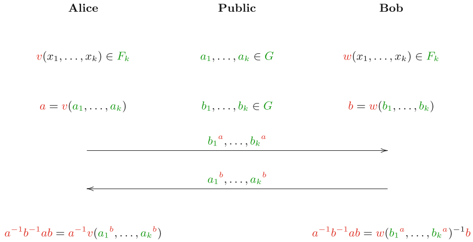
Fig. 1. The Commutator key exchange protocol
