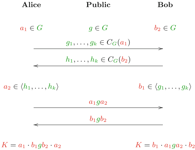
Fig. 2. The Centralizer key exchange protocol
