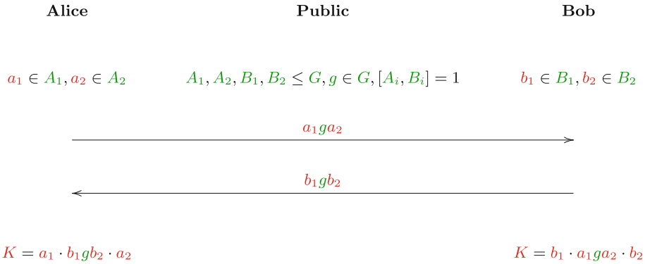
Fig. 4. The Double Coset key exchange protocol
