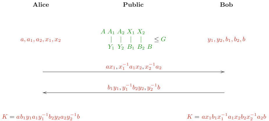
Fig. 6. The Triple Decomposition key exchange protocol
